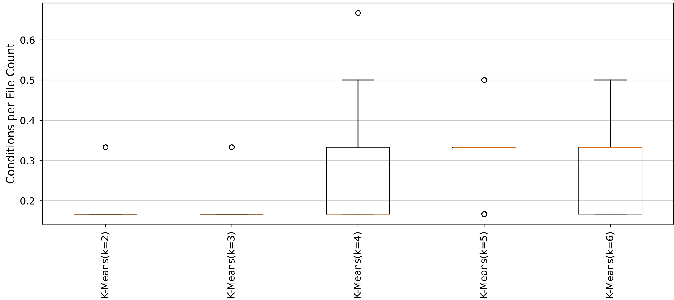
YARA Rules Conditions per File Count Distribution (Cluster28_Size6 dataset)
